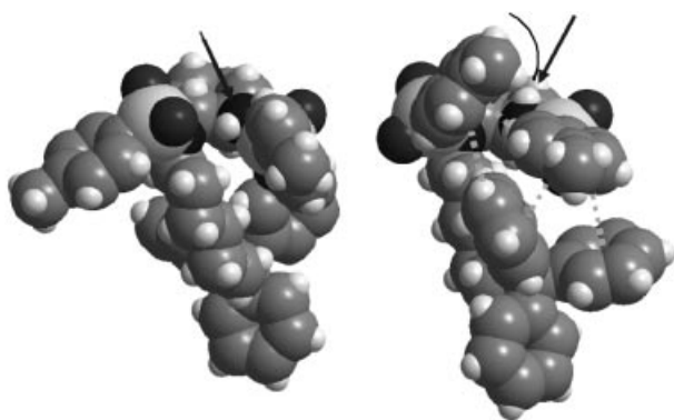
Figure 5. Global minima obtained for 2e with MMFF (left) and MMFFaq (right) force fields. An arrow points to the nonalkylated NH and possible aryl-aryl interactions are highlighted with dashed lines.
