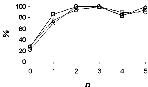
Figure 4. Plots of monoalkylation selectivity (squares) and fraction of folded conformations obtained by Monte Carlo searches (MMFF in circles and MMFFaq in triangles) versus the length of the alkyl chain ( n in Scheme 1).
