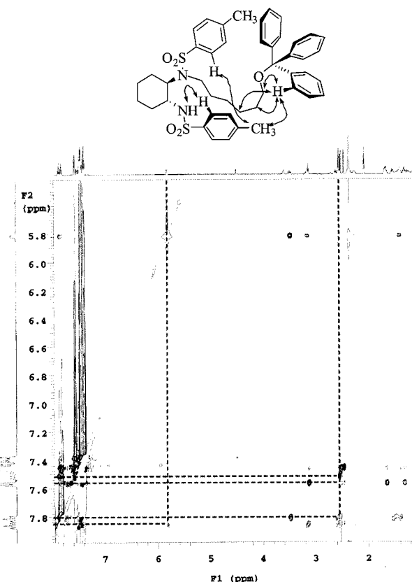
Figure 2. Selected NOE effects observed in the NOESY spectrum of ( R,R )- 2e ( \text{CD}_3\text{CN} , 500 MHz).
