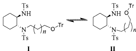
Figure 1. Proposed conformational equilibrium of the monoalkylated intermediate.
