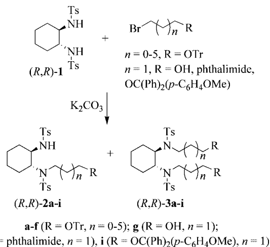
Scheme 1. Alkylation of bis(sulfonamide) ( R,R )- 1 .
