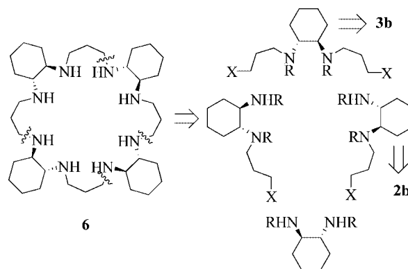
Scheme 3. Retrosynthetic analysis of macrocycle ( R,R,R,R,R,R,R,R )- 6 (R: protecting group, X: leaving group).
