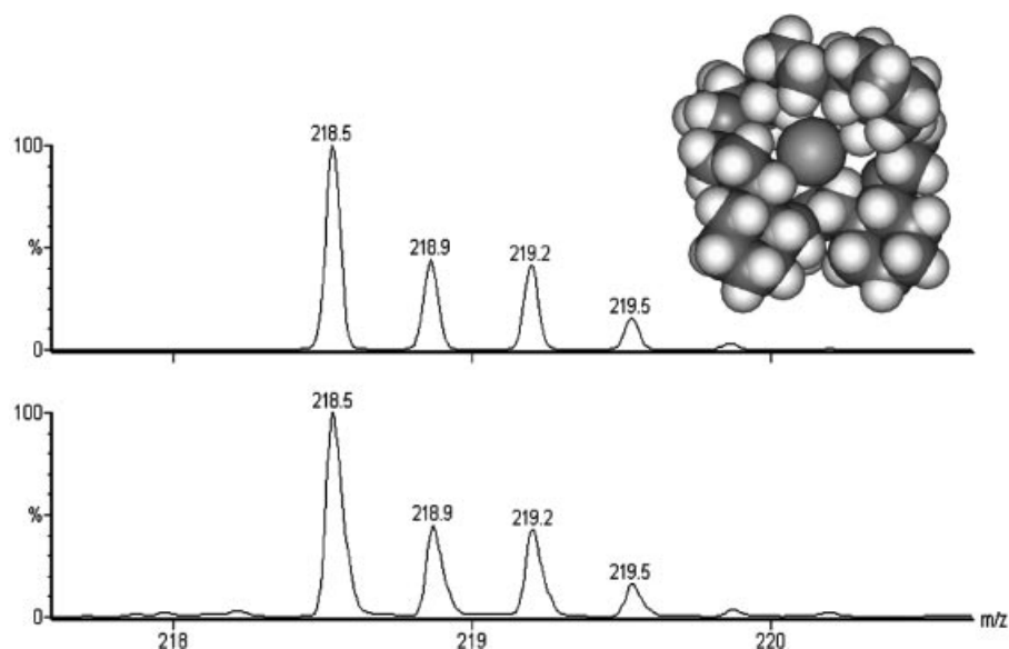
Figure 6. Experimental (lower trace) and simulated (upper trace) ESI-TOF spectra of an aqueous solution of the octahydrochloride of (R,R,R,R,R,R,R,R) - 6 , showing the base peak assigned to the [\mathbf{6} \cdot 4\text{H}^+ + \text{Cl}]^{3+} species. A molecular model (Monte Carlo simulation with MMFFaq minimizations) is also shown in CPK representation.
