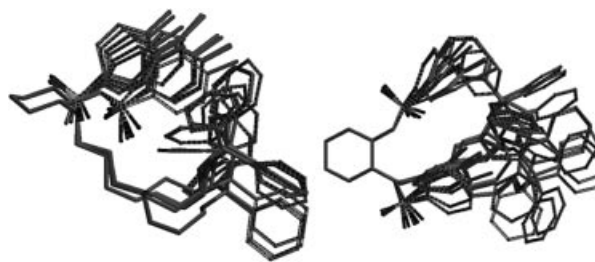
Figure 3. Side and upper views of superimposed conformations of 2f within an energy gap of 1 kcal/mol. Hydrogen atoms have been omitted for clarity.
