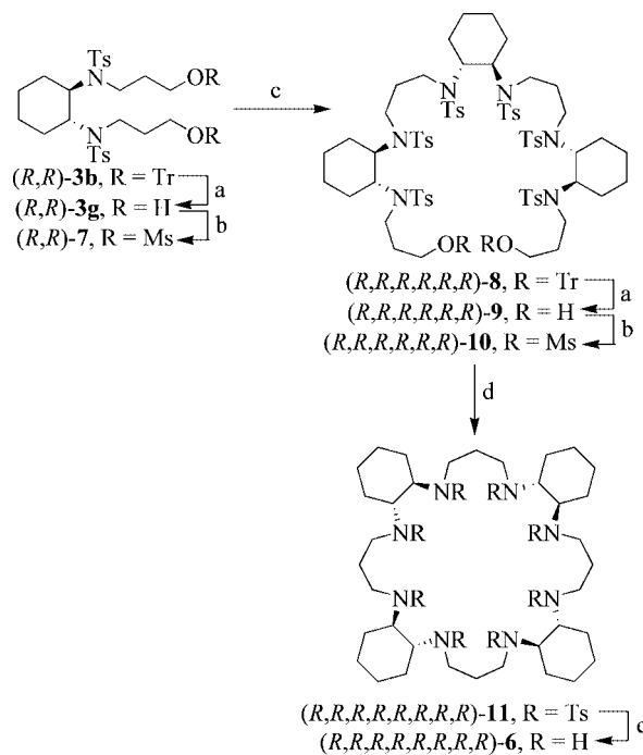
Scheme 4. Synthesis of macrocycle (R,R,R,R,R,R,R,R) - 6 . Reagents and conditions: a) TFA in \text{CH}_2\text{Cl}_2 :MeOH; b) MsCl/ \text{NEt}_3 in \text{CH}_2\text{Cl}_2 [60%, two steps from (R,R) - 3b ]; c) (R,R) - 2b , \text{Cs}_2\text{CO}_3 , \text{NBu}_4\text{Cl} cat., \text{PhCH}_3 (60%); d) (R,R) - 1 , \text{Cs}_2\text{CO}_3 , \text{CH}_3\text{CN} , (74%); e) HBr (aq.), PhOH, then NaOH with \text{CH}_2\text{Cl}_2 extraction and then HCl (85%).
